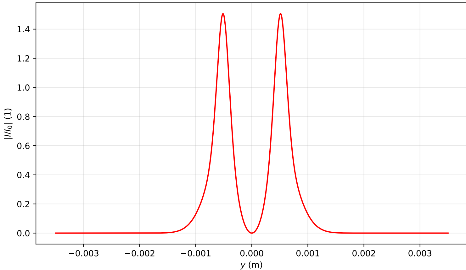
Intensity profile I(x=0, y, z=0.398)/I_0 , P_{in}=8.0P_{cr} , artificial time
